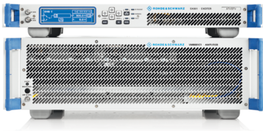
R&S®SCx8000 transmitter configured as R&S®SCW8601EA with an R&S®VM8601C1 VHF amplifier and an R&S®SX801 exciter. All VHF models have only one amplifier.
