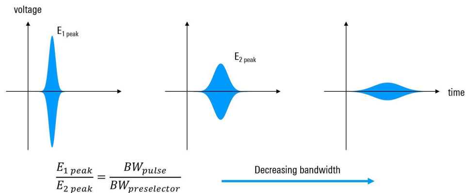
Figure 17 - Effect of preselector bandwidth on pulsed signal shape
