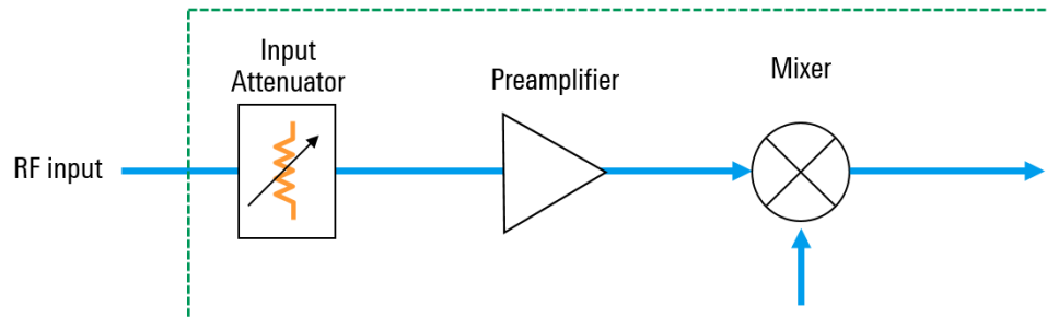
Figure 2 - Controlling mixer input level
