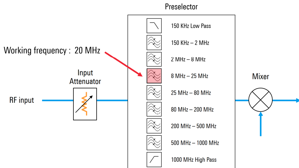
Figure 9 - Preselector concept
