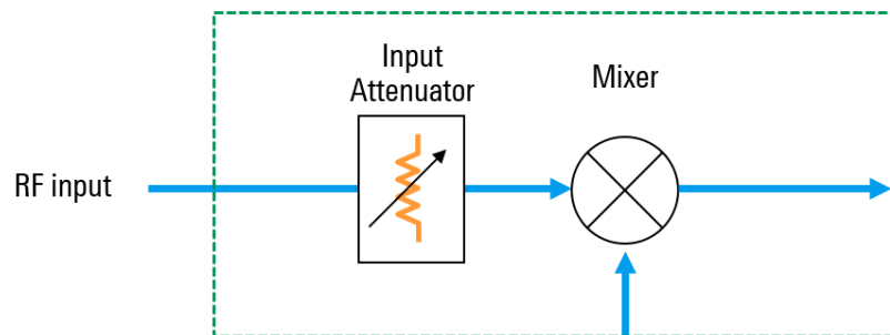
Figure 6 - Protecting the mixer with input attenuation
