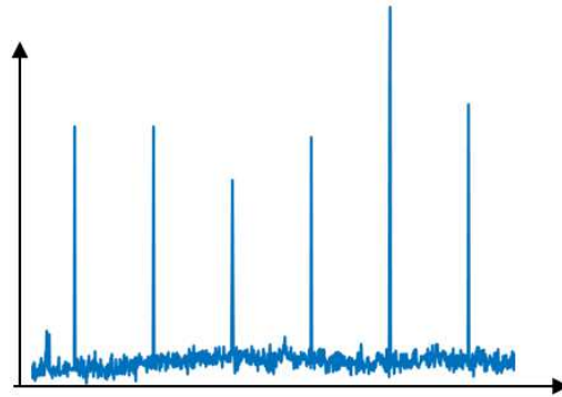
Figure 4 - Spurious products created by mixer compression
