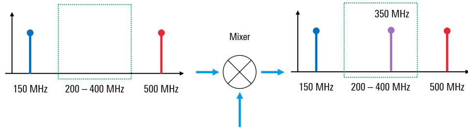
Figure 5 - Spurious product created in uncompressed mixer
