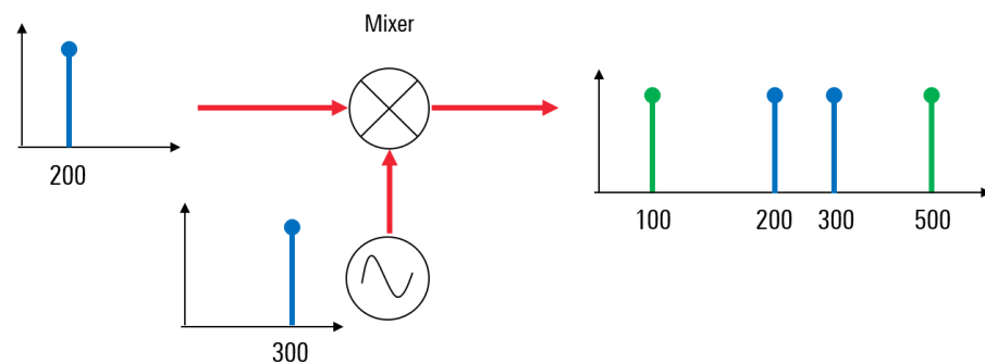
Figure 1 - Basic mixer principle
