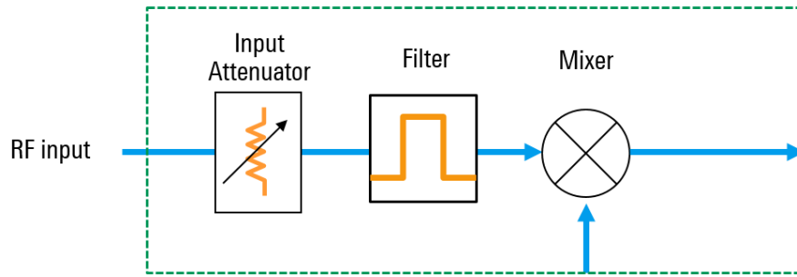
Figure 7 - Protecting the mixer with a (fixed) filter
