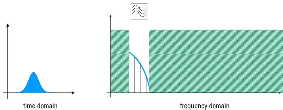
Figure 16 - Preselected pulse in the time and frequency domains
