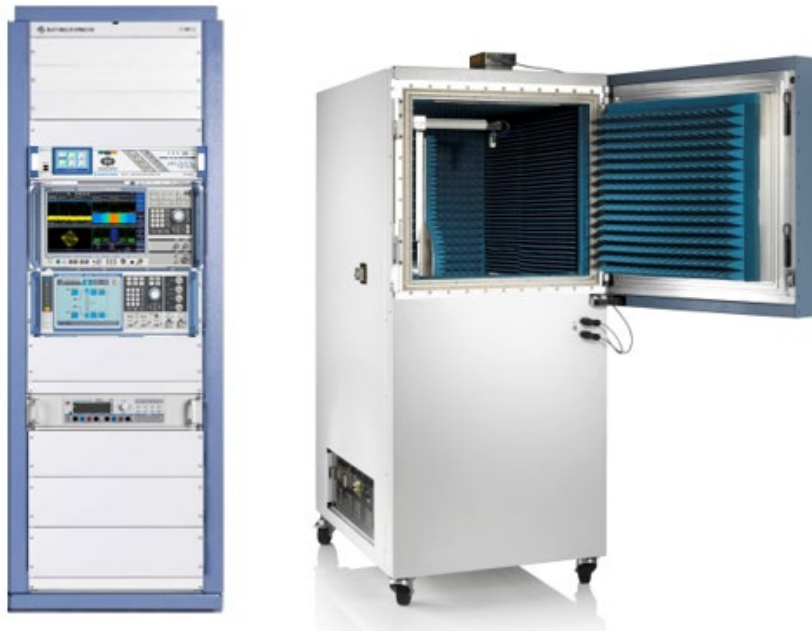
Fig. 3: Rohde & Schwarz mmWave OTA verification test system
