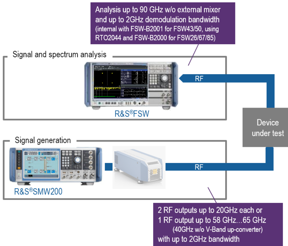
Fig. 2: Rohde & Schwarz 5G wideband solution
