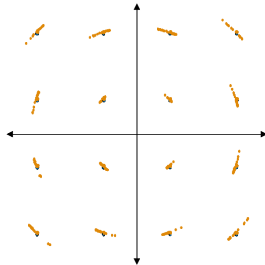
Figure 20 - Constellation with phase noise impairments
