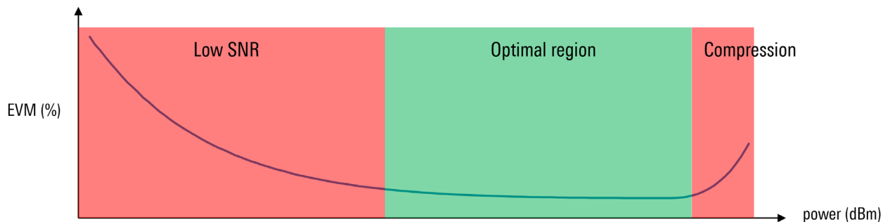
Figure 16 - EVM versus power
