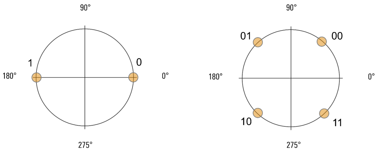
Figure 4 - BPSK and QPSK
