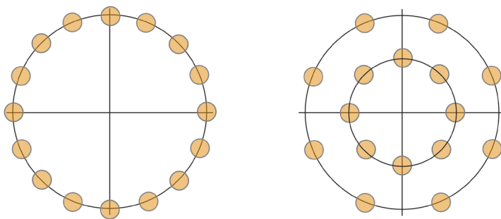
Figure 6 - 16PSK and 16APSK (two amplitude levels)
