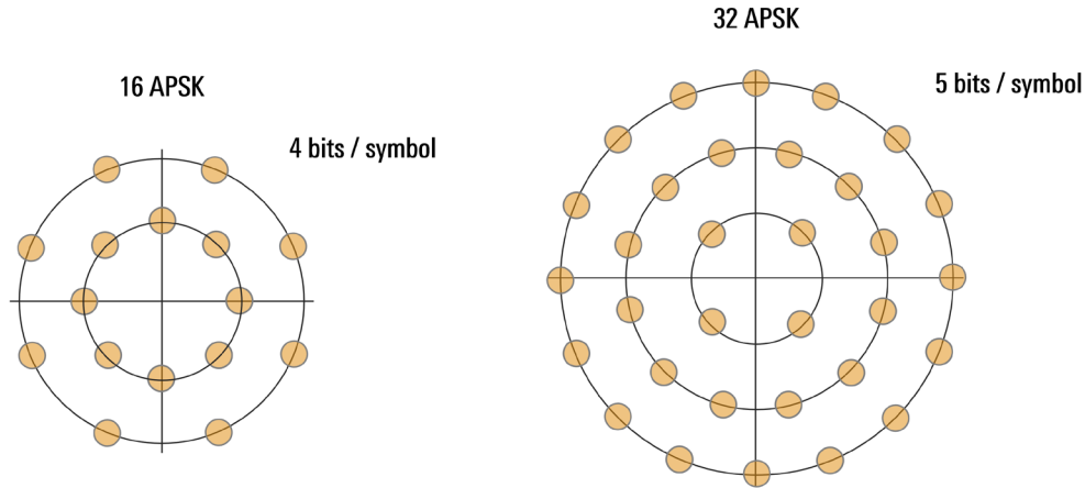
Figure 7 - 16APSK and 32APSK examples
