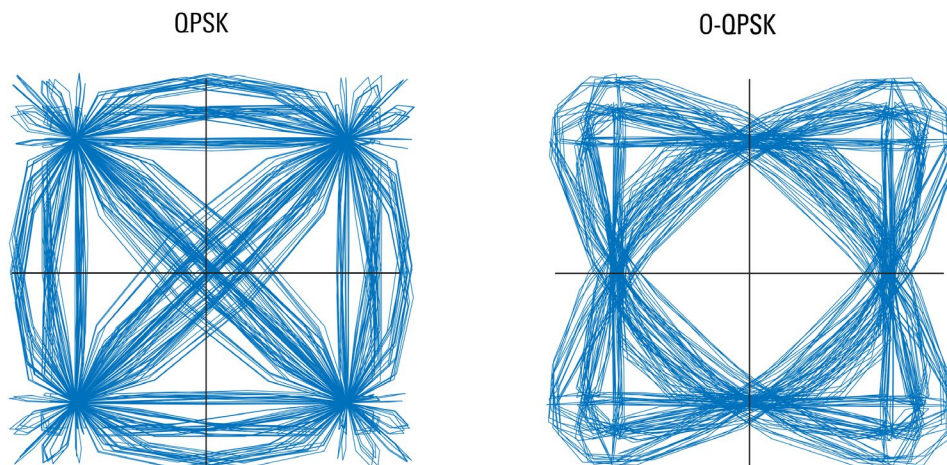
Figure 19 - Vector diagrams
