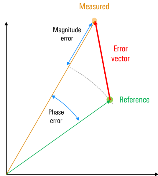
Figure 11 - Error vector
