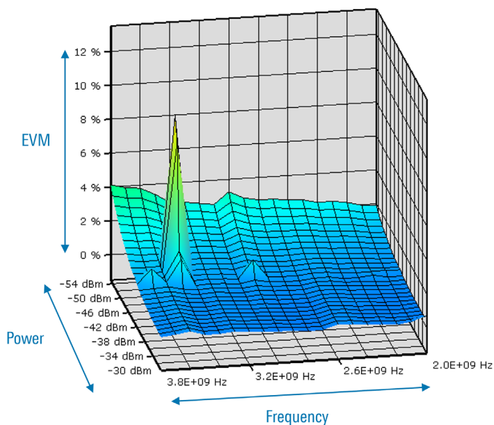
Figure 17 - EVM versus power and frequency
