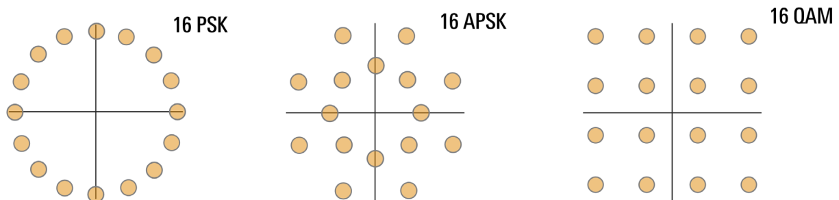
Figure 9 - Comparison of 16PSK, 16APSK, and 16QAM
