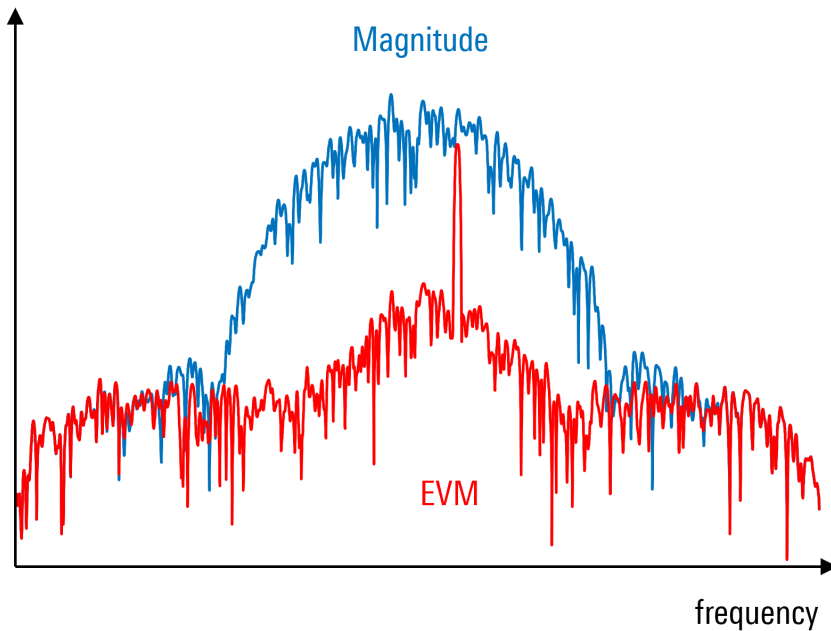
Figure 15 - EVM versus frequency
