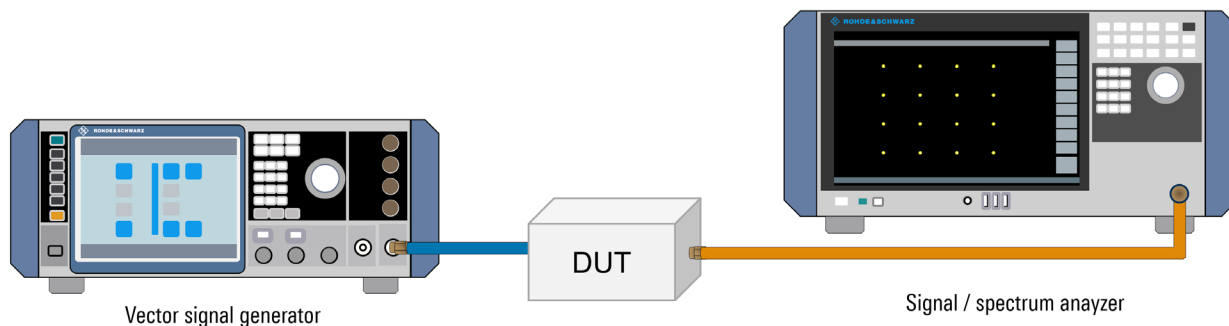
Figure 18 - EVM measurement setup
