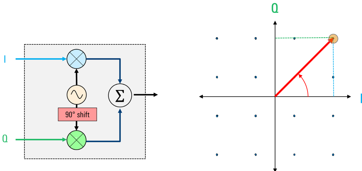
Figure 24 - IQ modulator and constellation diagram
