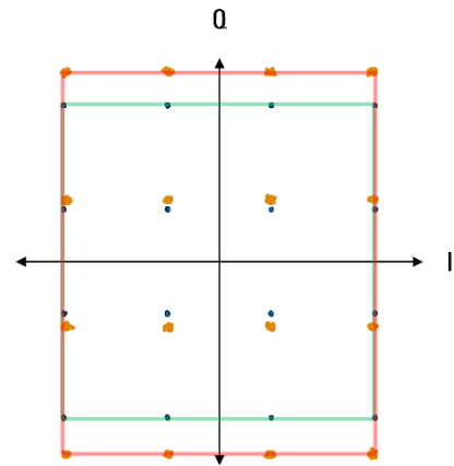
Figure 25 - IQ gain imbalance
