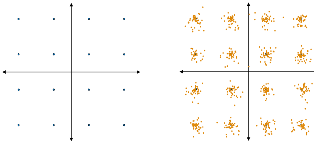
Figure 22 - High versus low SNR constellations
