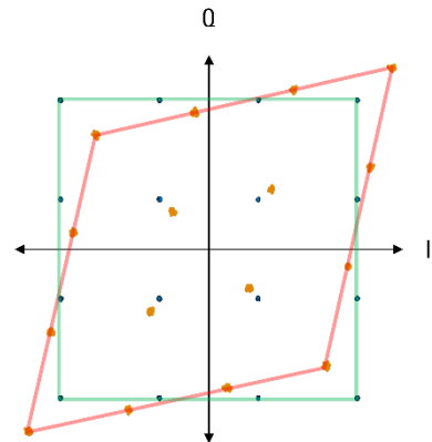
Figure 26 - IQ quadrature error
