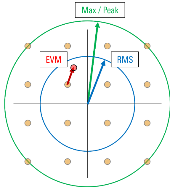
Figure 13 - Peak vs. RMS normalization of EVM
