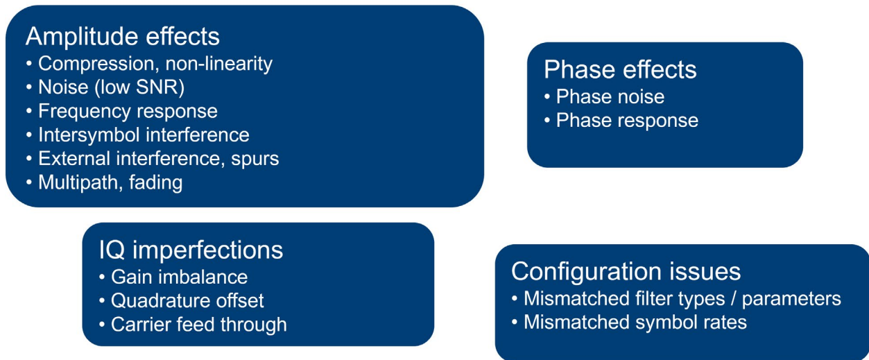
Figure 12 - Contributors to EVM
