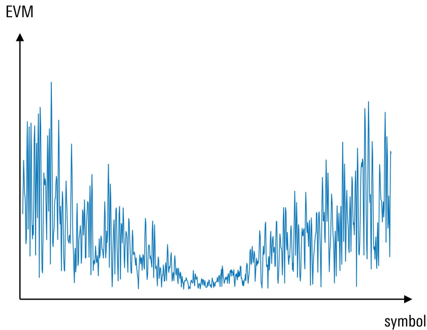
Figure 14 - EVM versus time / symbol
