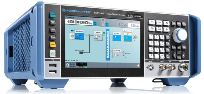
R&S®SMBV100B
