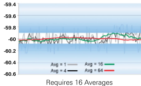
Sensor 2: -70 dBm Noise Floor
